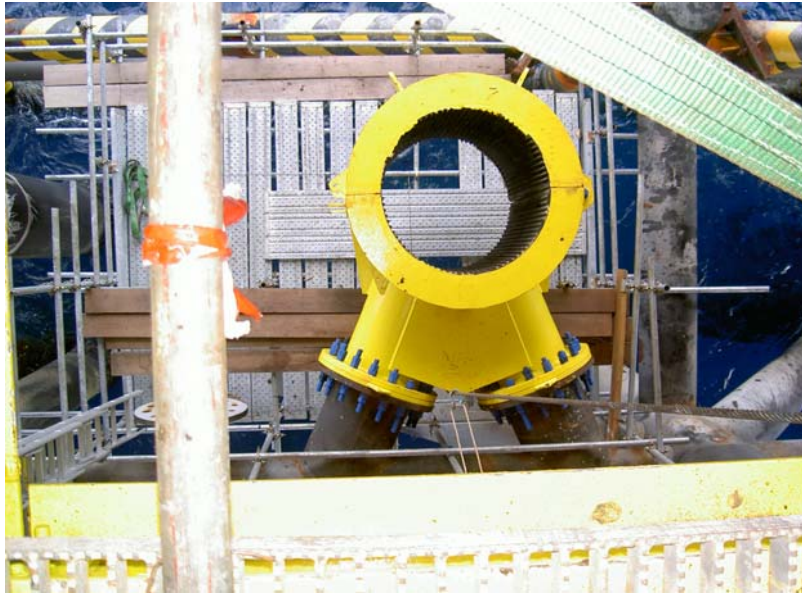
Completion of top riser clamp (+5 m) installation at CKR platform
