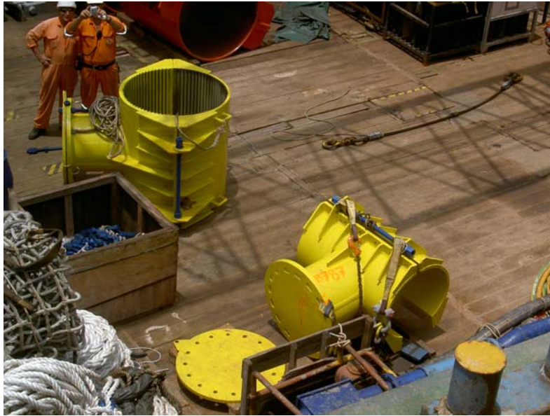
Riser clamp preparation (-9 m) for installation at CKR platform
