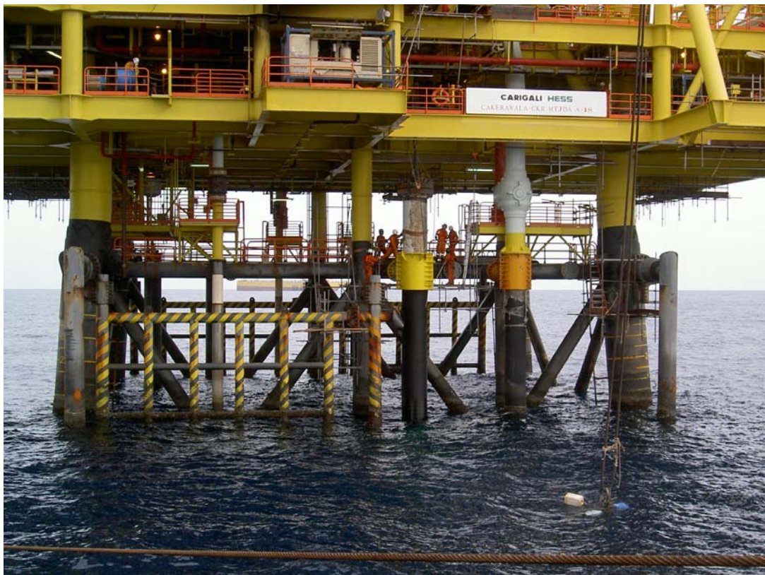
Riser installation at CKR platform
