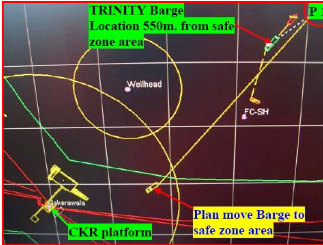
Pre-commissioning supporting vessel (Trinity Elbe) arrived in the field
